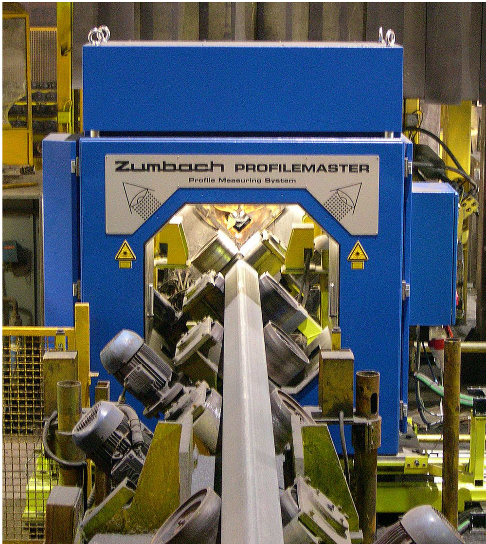
PROFILEMASTER® SPS 300 Measuring System
