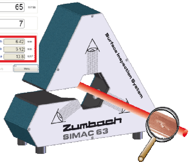
SIMAC ® 63 with typical display of the cameras and log of faults
