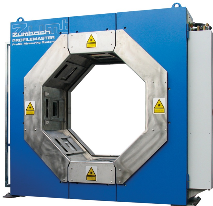
ZUMBACH's PROFILEMASTER® SPS 800 measuring unit
